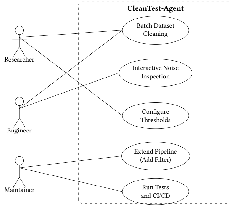
Fig. 1. UML Use Case Diagram
