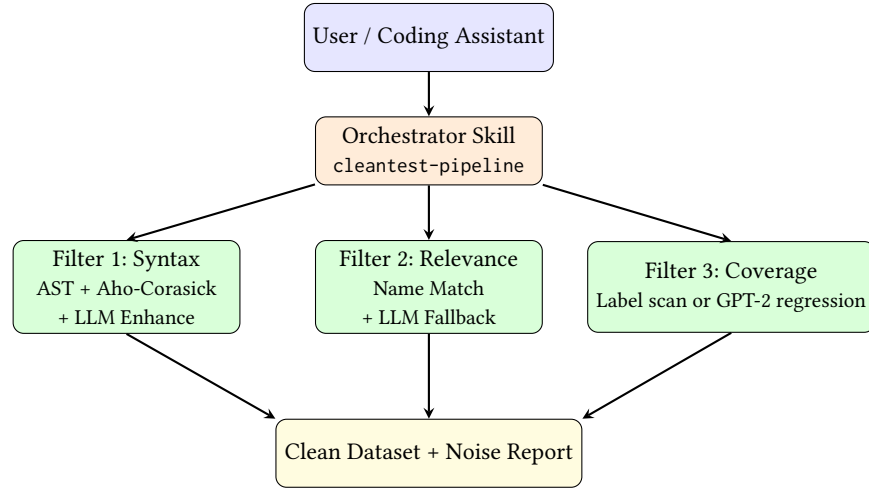
Fig. 4. CleanTest-Agent System Architecture
