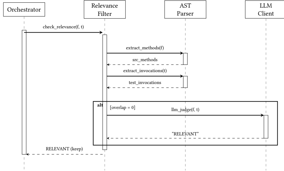
Fig. 3. Sequence Diagram: LLM-Enhanced Relevance Check
