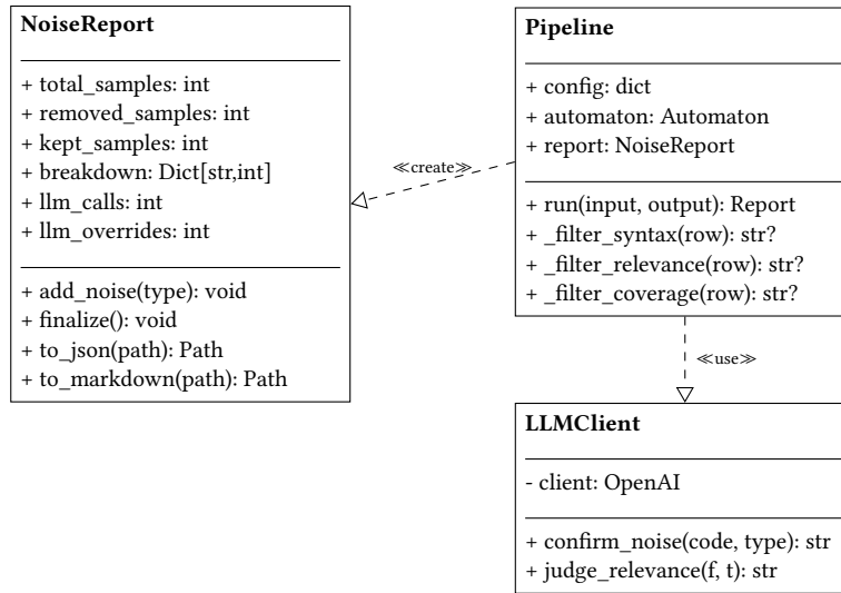
Fig. 6. Class Diagram: Core Data Types
