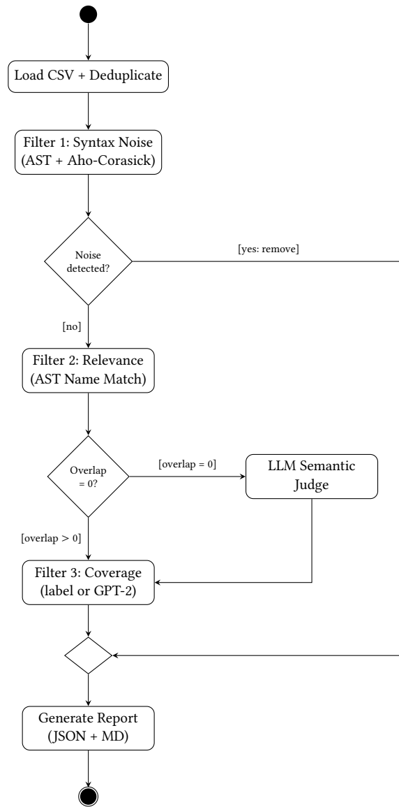
Fig. 2. Activity Diagram: Batch Cleaning Pipeline (UC1)
